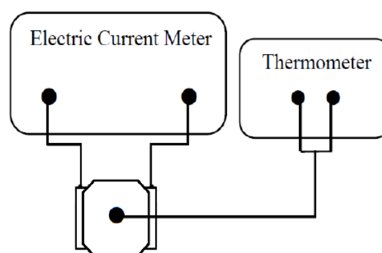
Irms test schematic diagram
