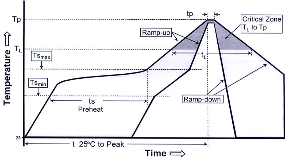
标准回流焊曲线 Standard soldering profile
