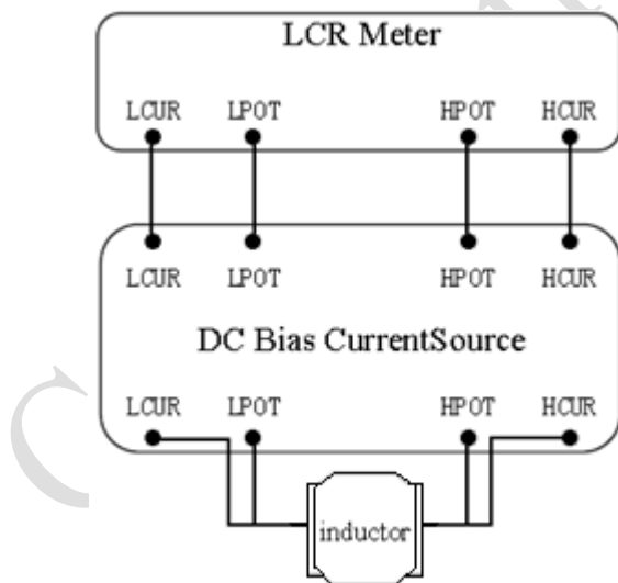
Isat test schematic diagram
